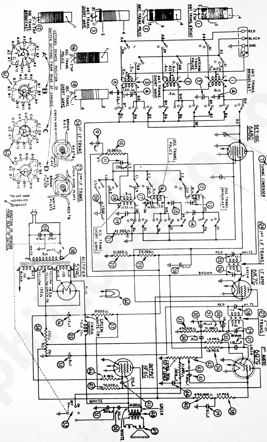
Fig. 5—Schematic Diagram—Model 37-610
