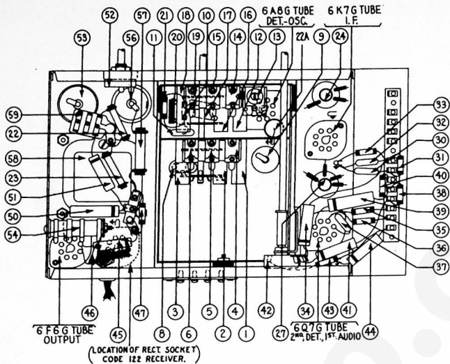
Fig. 6—Base View of Chassis
