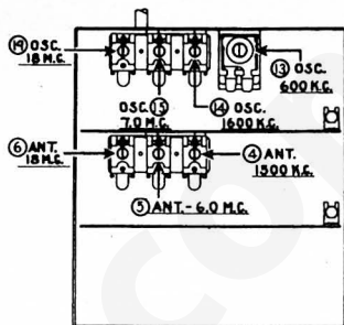
Fig. 4—Locations of R.F. Compensators Underside of Chassis
