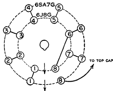
TYPE 6J8G 6A8G REPLACING TYPE 6SA7GT TYPE 12K8G REPLACING TYPE 12SA7GT
