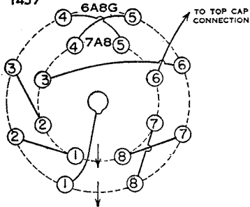
TYPE 7A8 14B8 REPLACING TYPE 12A8GT 14J7 REPLACING TYPE 12K8G
