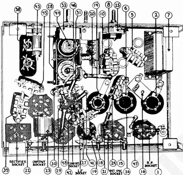
Bottom View of Chassis, Showing Parts
