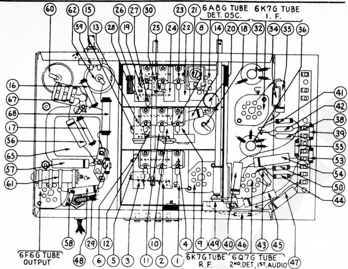
Fig. 6—Base View
