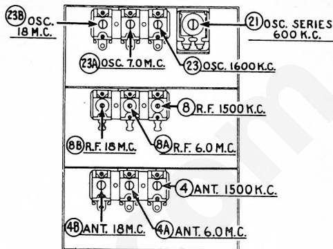
Fig. 4—Locations of R. F. Compensators
