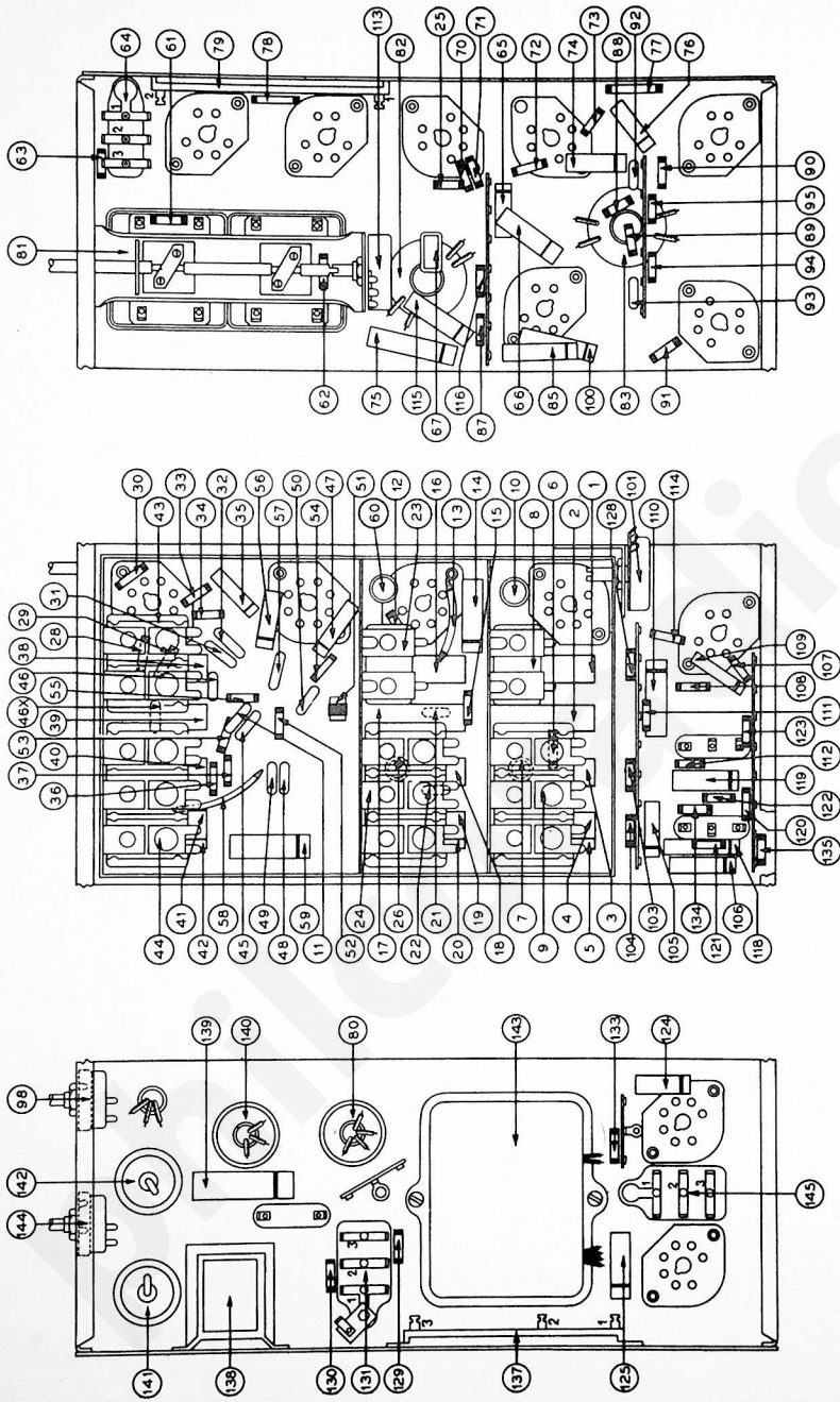
Fig. 2. Underside View of Chassis
