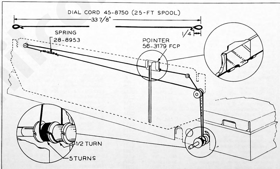
Figure 5. Drive-Cord Installation Details
