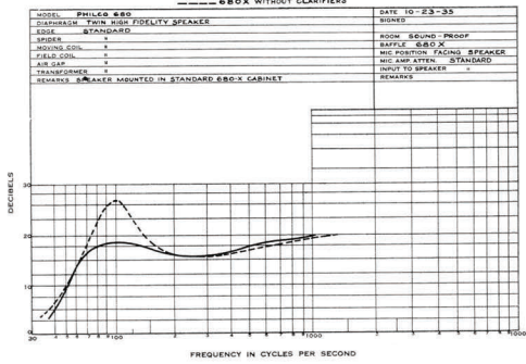
Philco Acoustic Clarifiers prevent cabinet resonance
