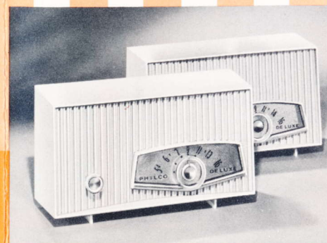
PHILCO 822. High sensitivity with Philco's new "Clip-In" chassis. 4 tubes plus rectifier. Built-in loop antenna. Lustre Ivory or Lemon Yellow. 6 \frac{1}{8} " High, 11 \frac{3}{4} " Wide, 4 \frac{1}{4} " Deep.
