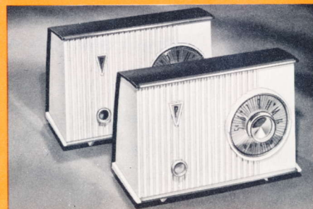
PHILCO 824. "Slender Set" full dress styling finished front and back. New "Clip-In" chassis. Lustre Ivory or Pink with Ebony and Gold trim. 7 \frac{3}{4} " High, 10 \frac{3}{4} " Wide, 4 \frac{1}{2} " Deep.
