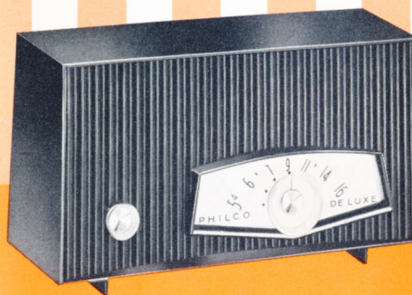
PHILCO 820. "Slender Set" styling in Mahogany finish. New "Clip-In" chassis with 4 tubes plus rectifier. Big, extra sensitive 4-inch speaker. 6 \frac{1}{8} " High, 11 \frac{3}{4} " Wide, 4 \frac{1}{4} " Deep.
