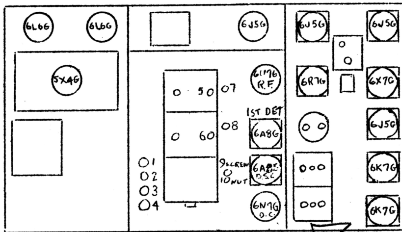
FRONT OF CHASSIS
