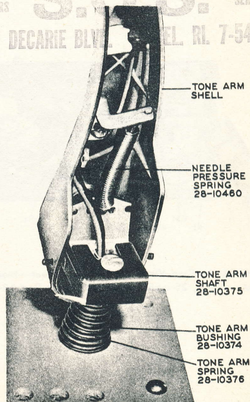
FIGURE 1—Tone Arm Assembly Mounting
