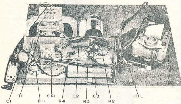
FIGURE 3—Base View, Components Layout—Model 832
