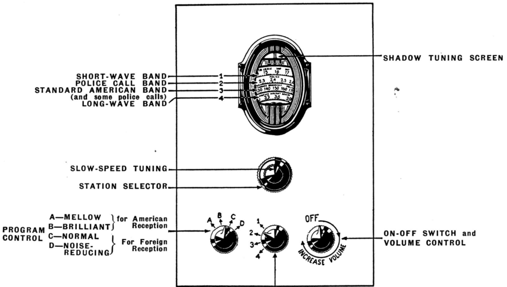
WAVE BAND INDICATOR AND AUTOMATIC AERIAL SELECTOR Locations of Controls, Model 650
