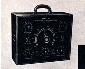
UHF Auto-Level Sweep Generator Model G-8002. The newest, most modern, most inexpensive UHF sweep generator on the market. Checks sweep alignment with any test oscilloscope. Its output is controllable... makes possible over-all trouble shooting and testing of low level units such as UHF tuners, boosters, converters, etc.
