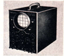
5-inch High Gain Oscilloscope Model S-8202. This outstanding scope is built to the highest standards of test instruments... It features the highest gain 10 millivolts/inch, and widest frequency range at its popular price. Wide sweep ranges allow flexibility in sweep circuit trouble shooting.
