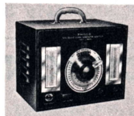
VHF to UHF Signal Generator Adapter Model G-8000. The most economical system yet designed to produce UHF signals for TV receiver tests. Through a conversion process this unit produces from an input VHF signal, UHF signals having the same characteristics as the VHF signal.
