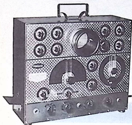
The Philco Visual Alignment Generator
