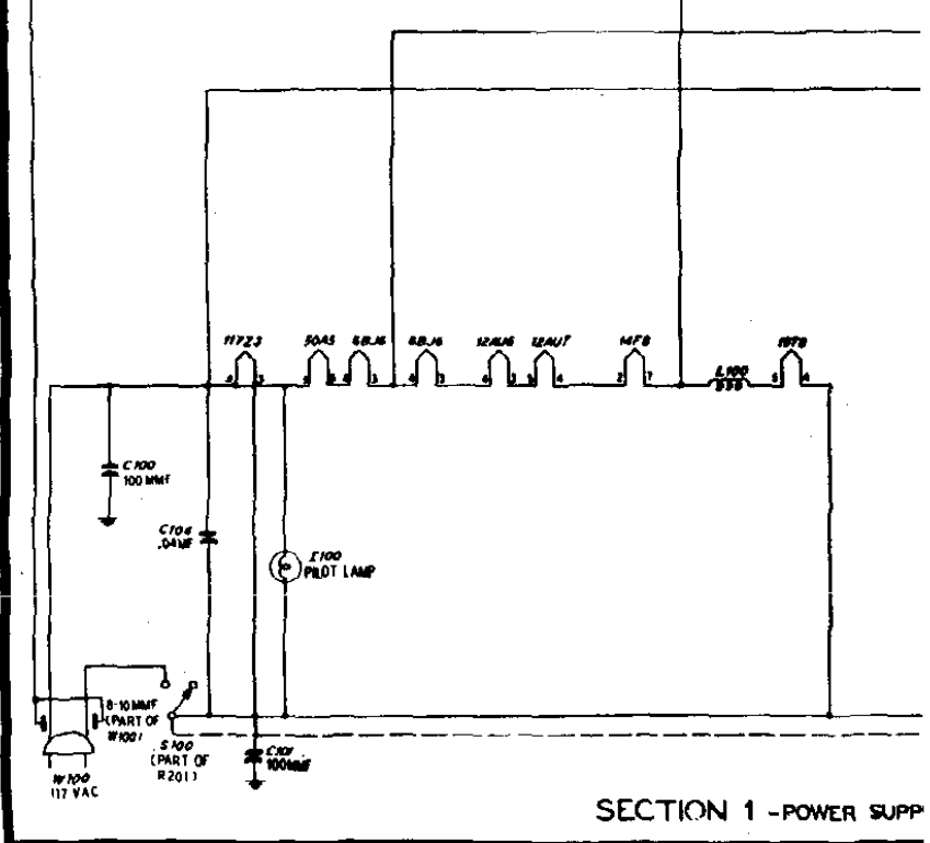
Figure 6. Philco Radio Model 48-472, Code 122.
