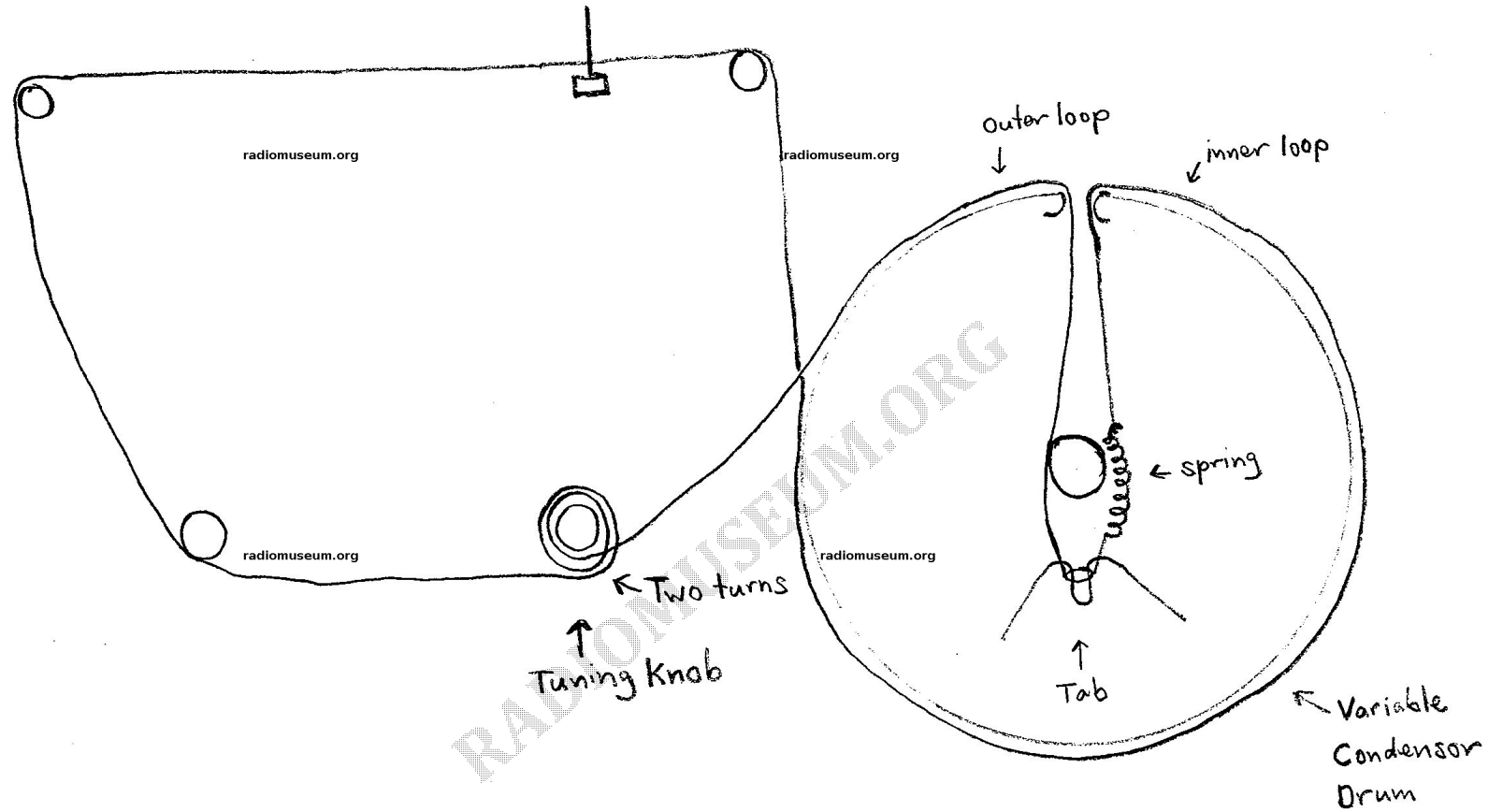
Dial Cord Diagram General Electric Models L-640 and L-641 Table Radios (1941)
