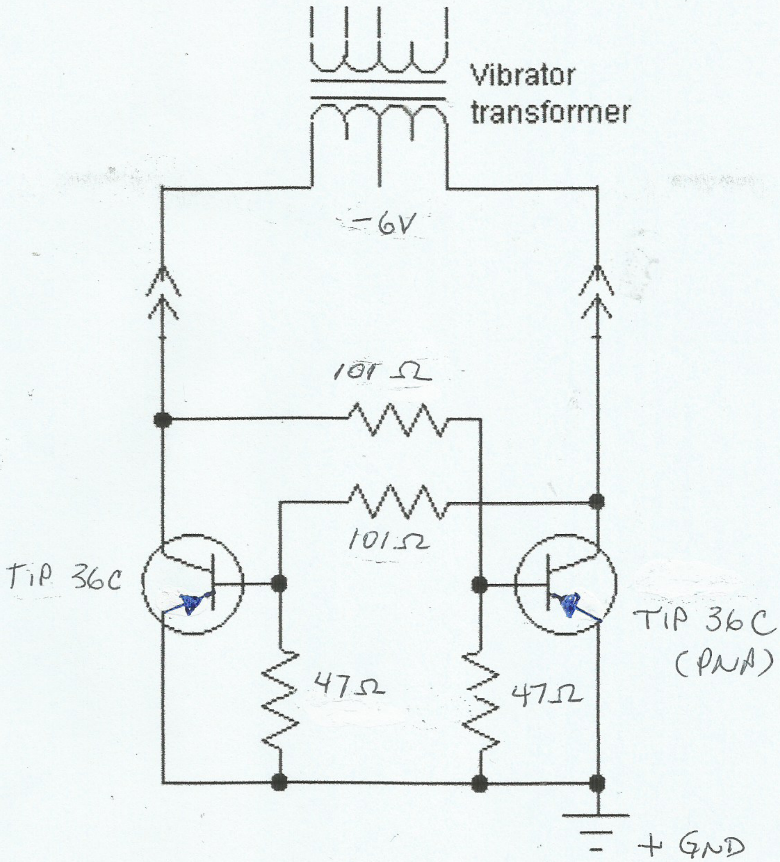
6V , + GND ASYNCHRONOUS VIBRATOR
