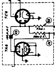
SCHEMATIC DIAGRAM MODEL 41-295, 41-300
