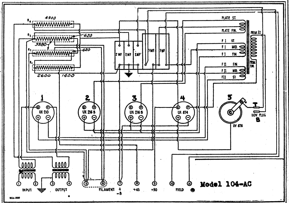
Terminal Layout
