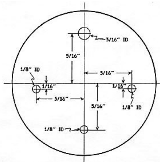
Fig. 2. Layout of drilling template for WD-11 base.
