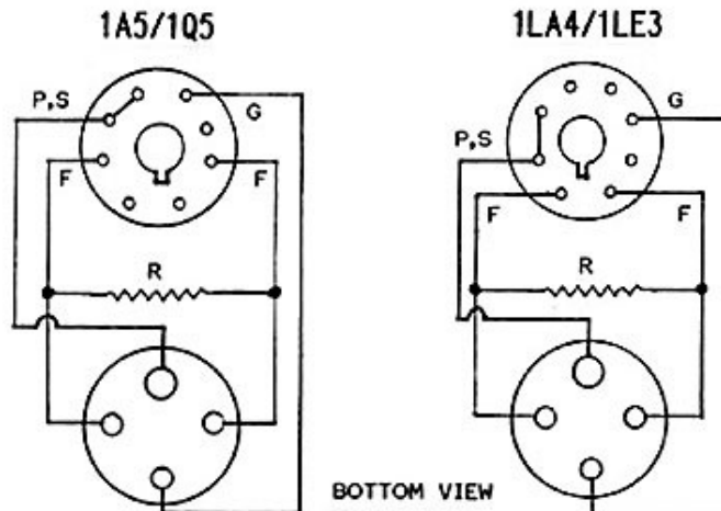
Fig. 4. Wiring diagrams for adapters. See text for function of resistor "R."
