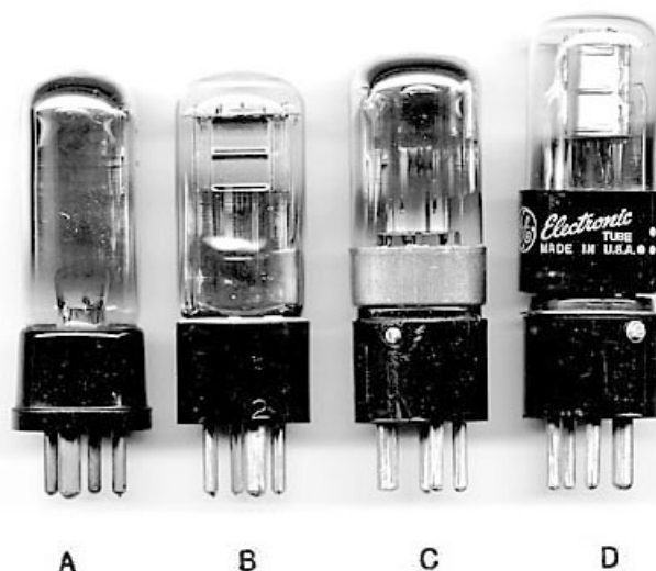
Fig. 5. From left: WD-11 tube; re-based 864; 1LE3 in its adapter; 1A5 in its adapter.
