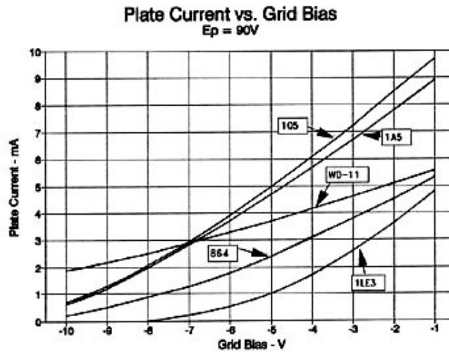
Fig. 1. Transfer characteristics of the WD-11, 864, and possible substitutes.
