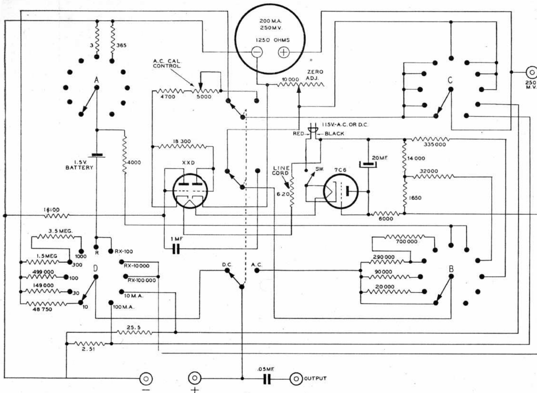
PHILCO MODEL 020 VOLT-OHMMETER (SCHEMATIC DIAGRAM)
