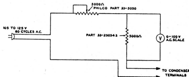
EXTERNAL CIRCUIT FOR CAPACITY METER
